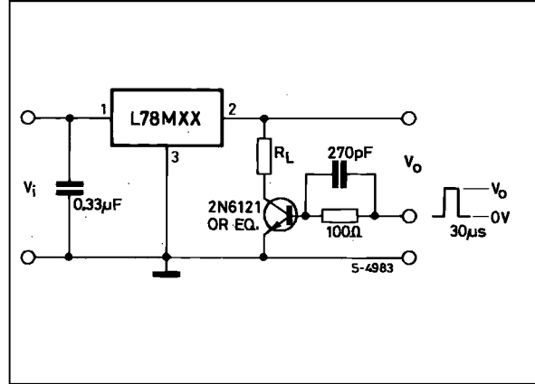
Figure 2 : Load Regulation.
