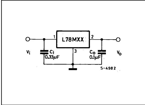
Figure 1 : DC Parameters.
